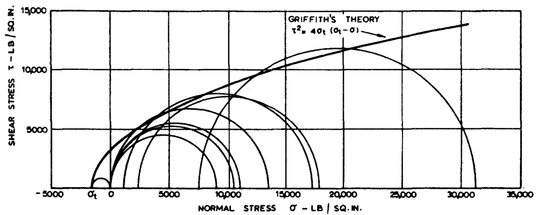
Figure 5. Mohr circles for fracture initiation at the boundary of an open crack.
