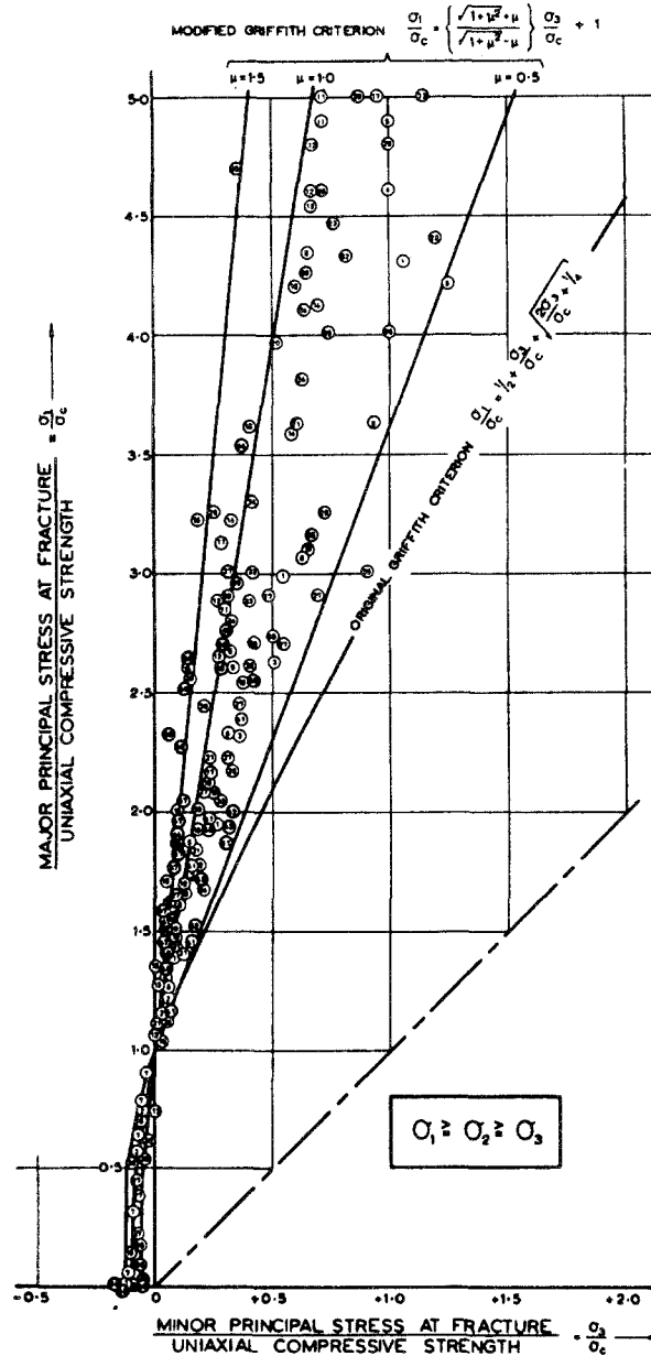
Figure 2. Triaxial fracture data for rock materials.
