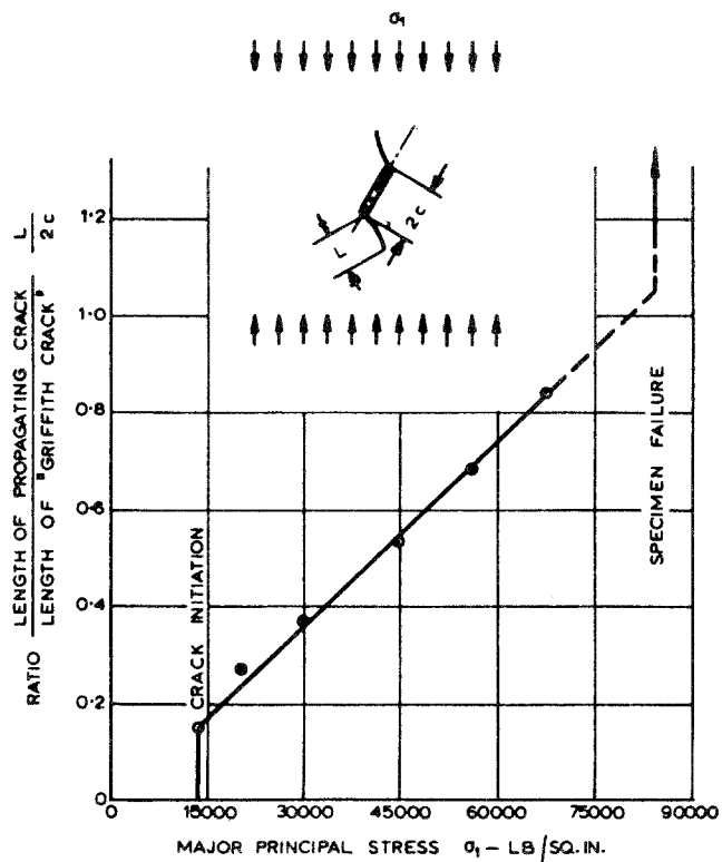
Figure 7. Relationship between propagating crack length and applied uniaxial compressive stress.
