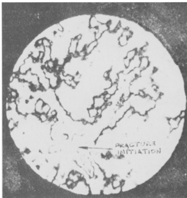
Figure 9. Reflected light photoelastic pattern showing strain distribution in a large grained granite plate subjected to uniaxial compression.
