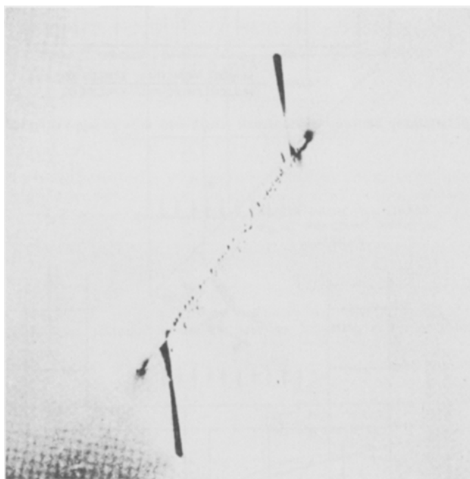
Figure 8. Fracture propagating from a closed crack in glass.
