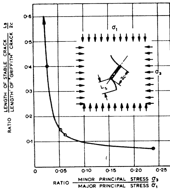
Figure 6. Relationship between stable crack length and ratio of applied principal stresses.
